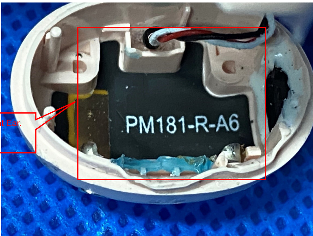
Antenna view of EUT
