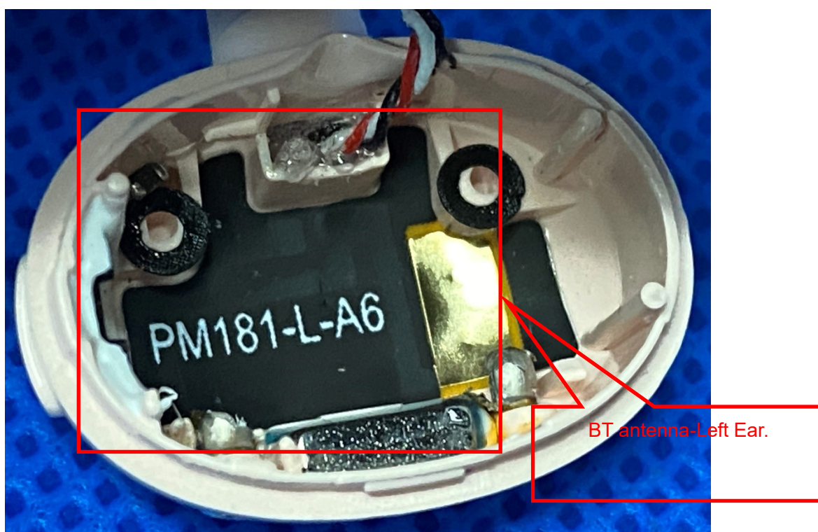
Antenna view of EUT
