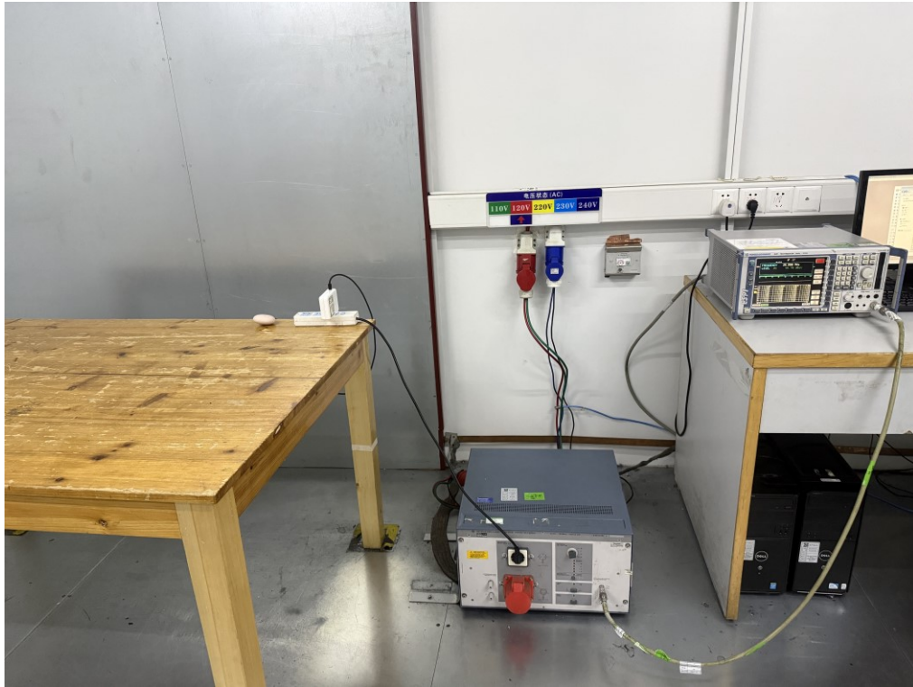
AC POWER LINE CONDUCTED TEST SETUP
