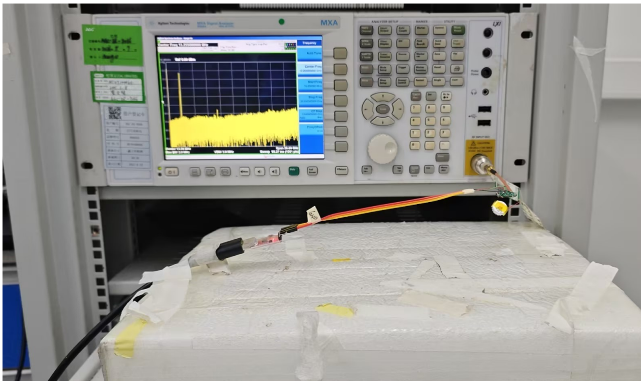
RF CONDUCTED TEST SETUP
