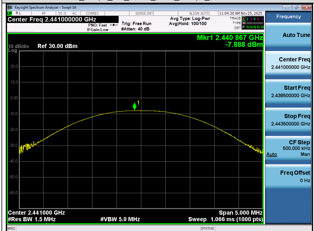
Test_Graph_BR_ANT1_2441_1Mbps_Peak Power
