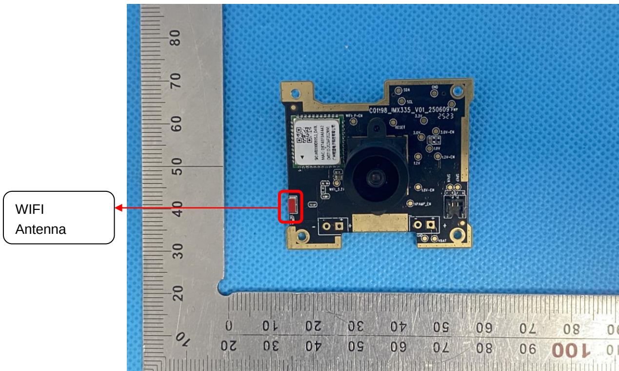
INTERNAL VIEW OF EUT(FIGURE 12)
