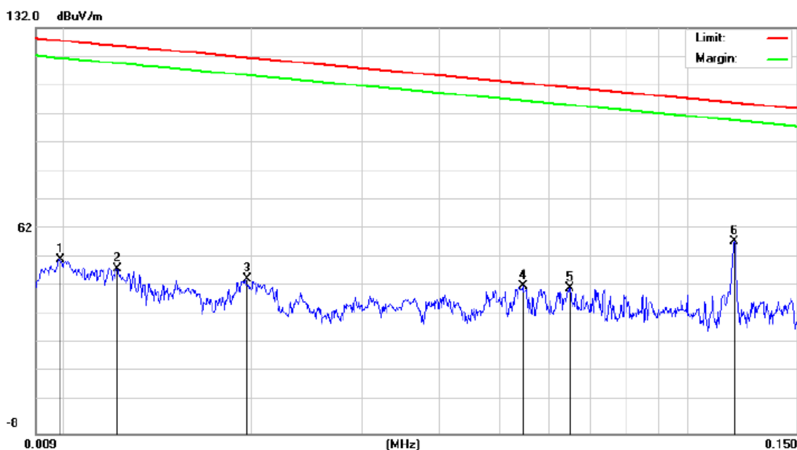
Test graph and data for Electric Field strength between 9kHz-150kHz
