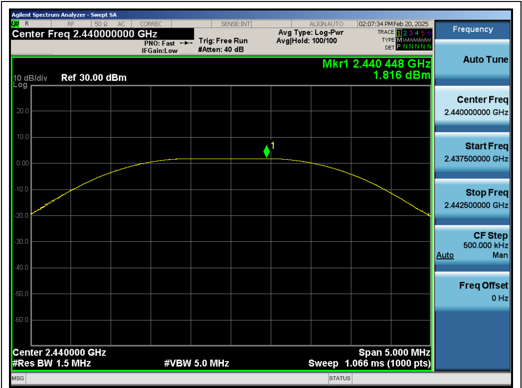
Test_Graph_LE2M_ANT1_2440_2Mbps_Peak Power
