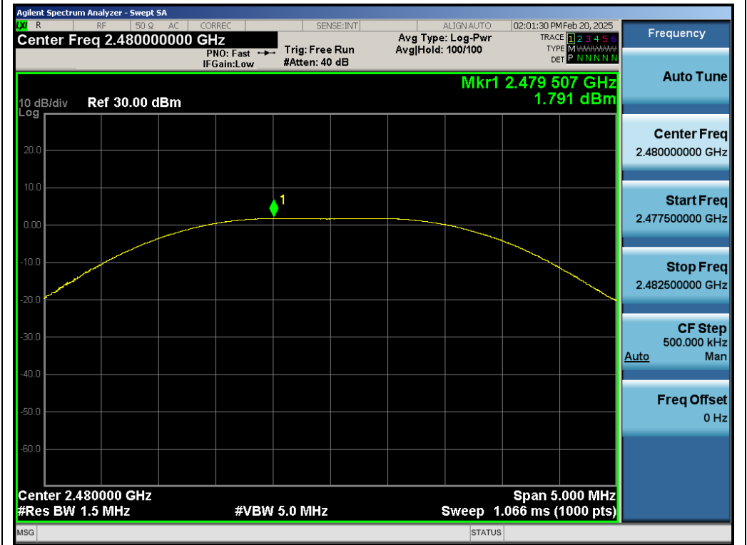
Test_Graph_LE2M_ANT1_2480_2Mbps_Peak Power
