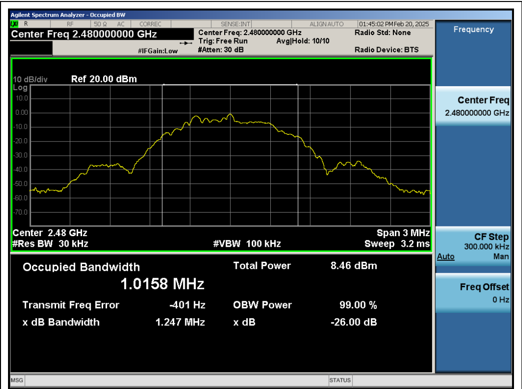
Test_Graph_LE1M_ANT1_2480_1Mbps_OBW
