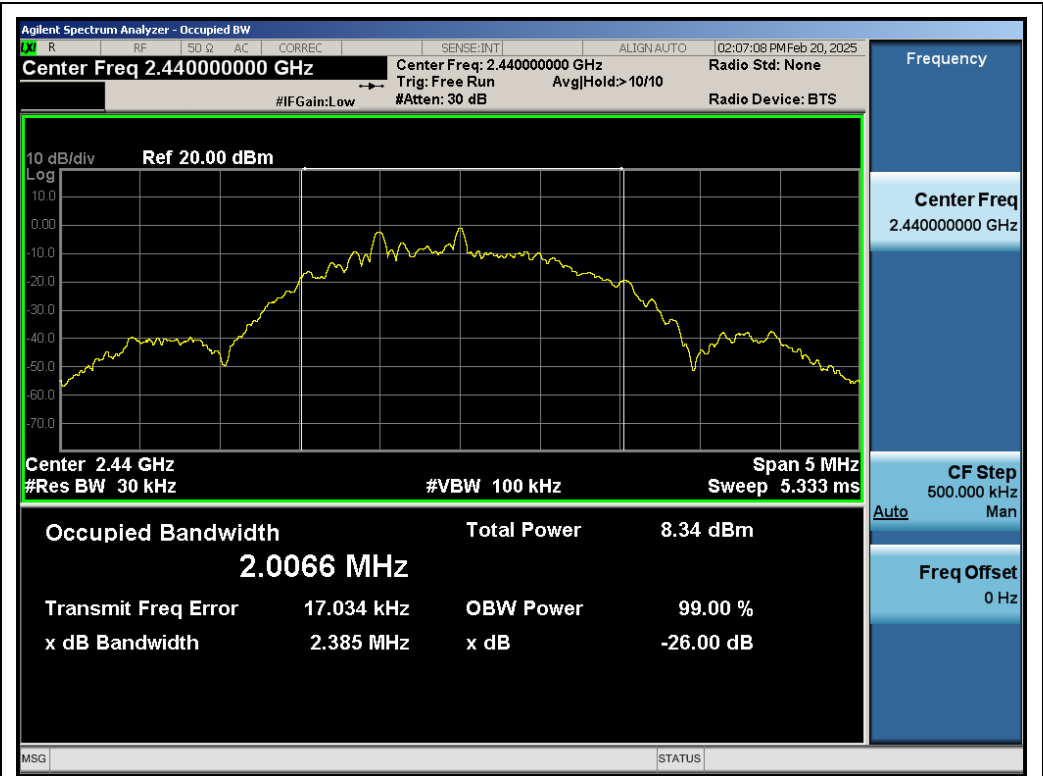
Test_Graph_LE2M_ANT1_2440_2Mbps_OBW
