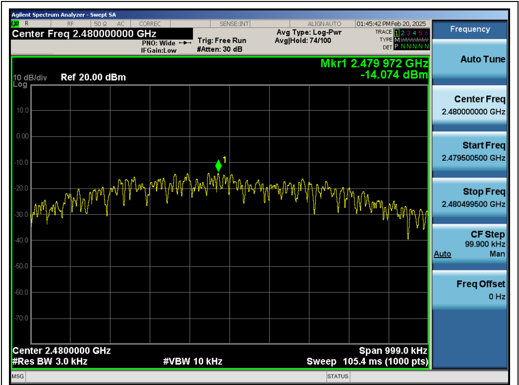
Test_Graph_LE1M_ANT1_2480_1Mbps_PSD
