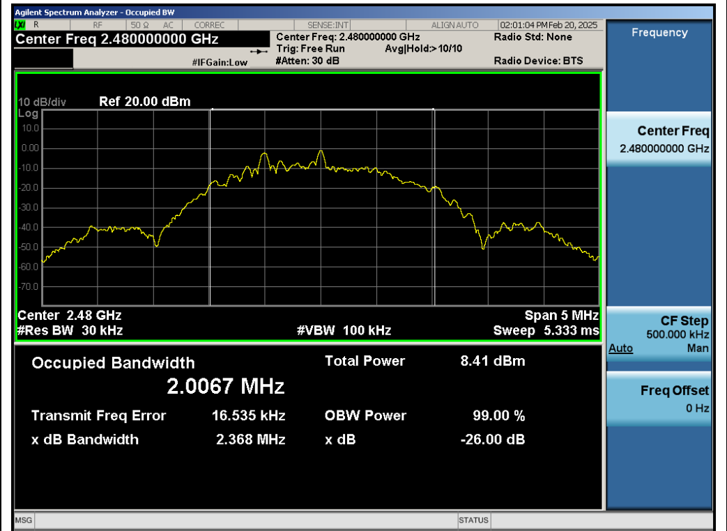
Test_Graph_LE2M_ANT1_2480_2Mbps_OBW
