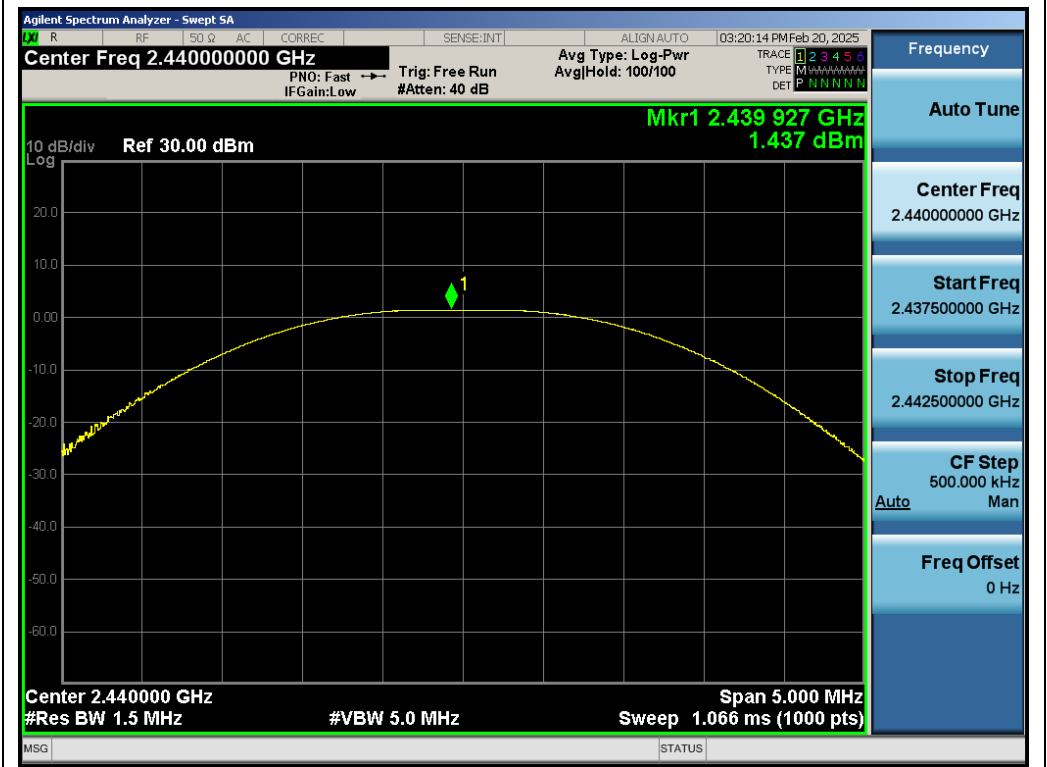
Test_Graph_LE1M_ANT1_2440_1Mbps_Peak Power
