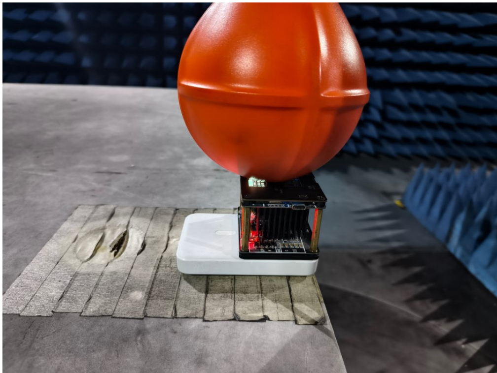
RF HEALTH ASSESSMENT TEST PHOTOS (0cm) Measure Position E
