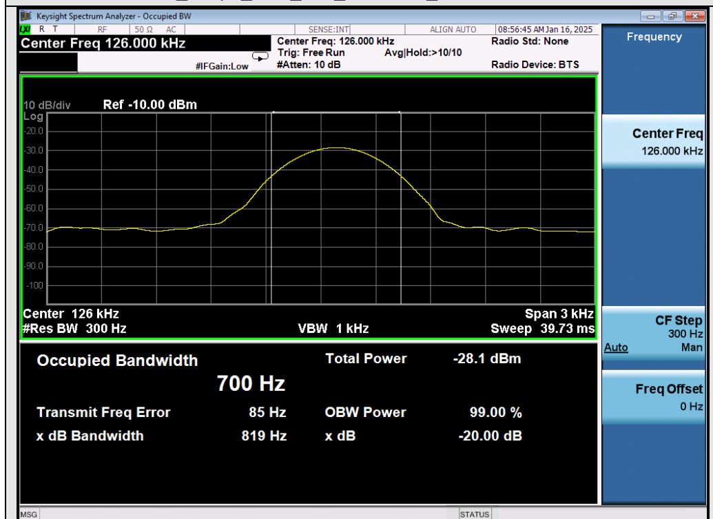
Test_Graph_ASK_Coil_126kHz_-20dB Bandwidth
