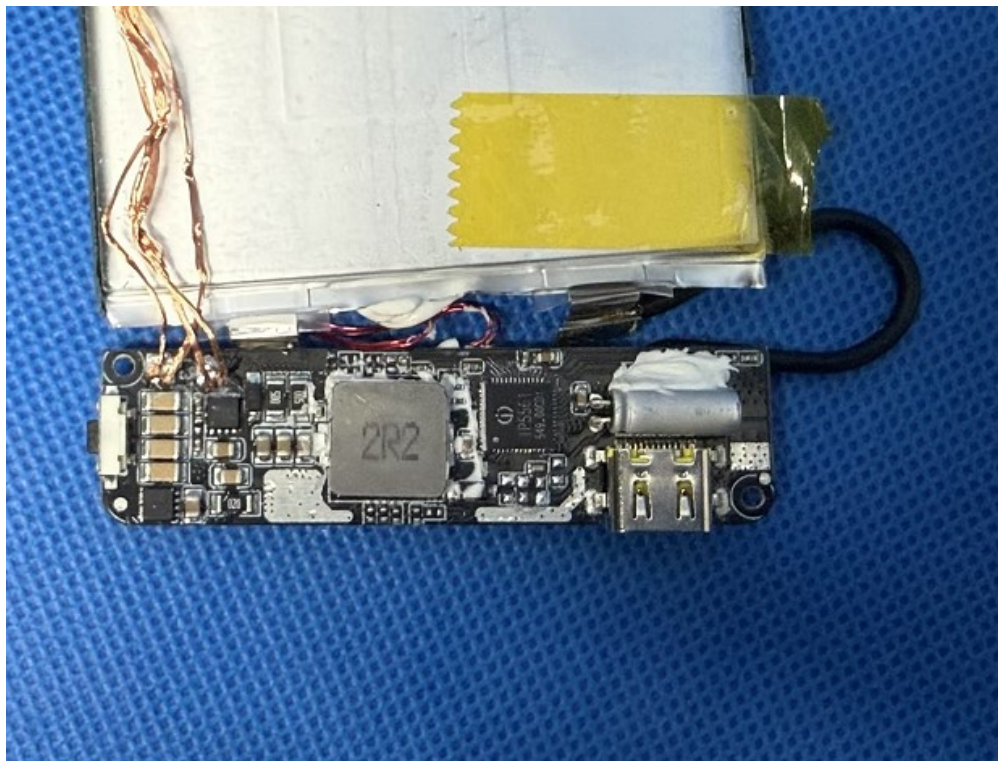
INTERNAL VIEW OF EUT (FIGURE 10) _With lithium battery protection circuitry
