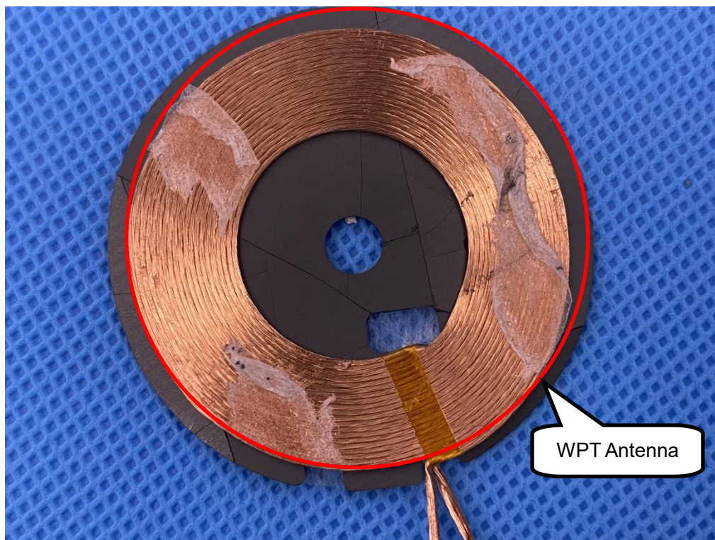
INTERNAL VIEW OF EUT (FIGURE 6) _Without lithium battery protection circuitry
