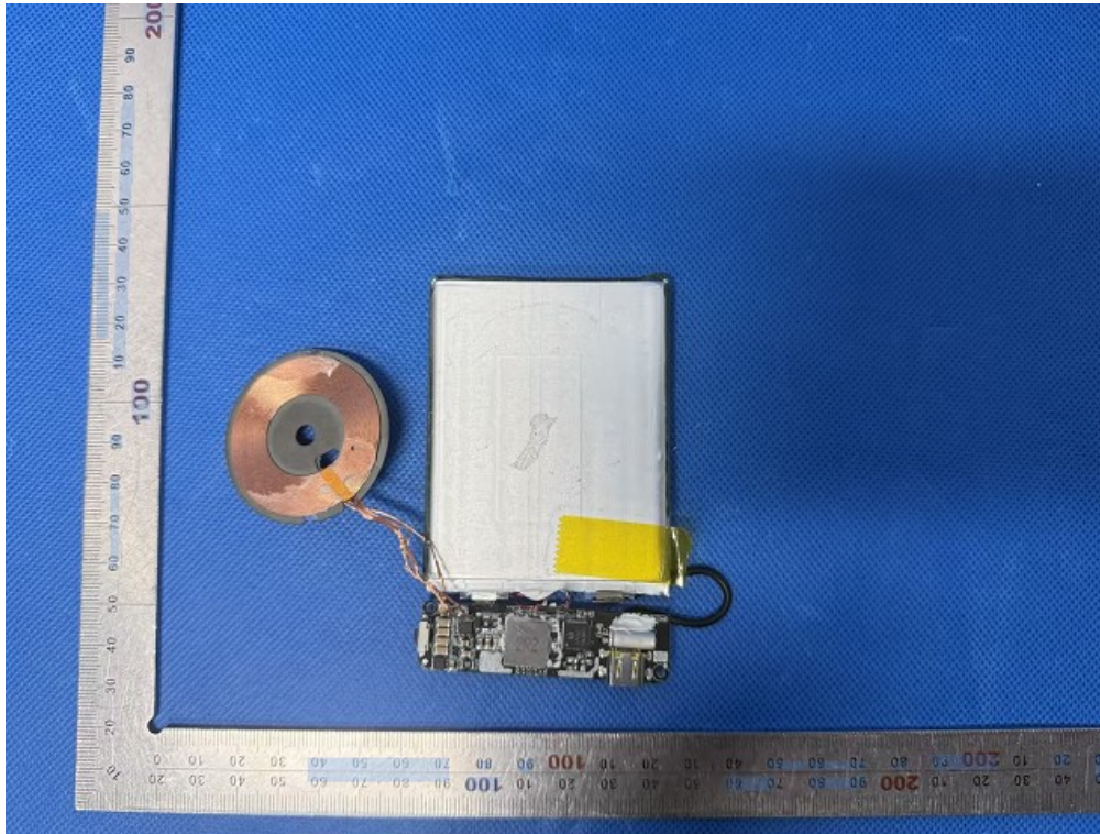
INTERNAL VIEW OF EUT (FIGURE 8) _With lithium battery protection circuitry
