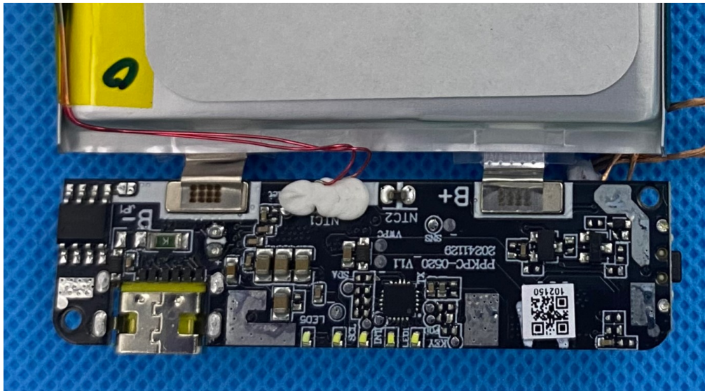
INTERNAL VIEW OF EUT (FIGURE 6) _Without lithium battery protection circuitry
