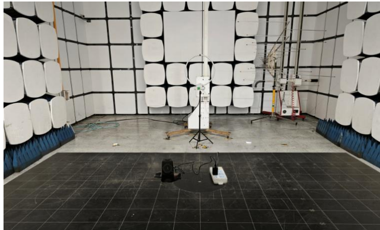
Radiated emission
