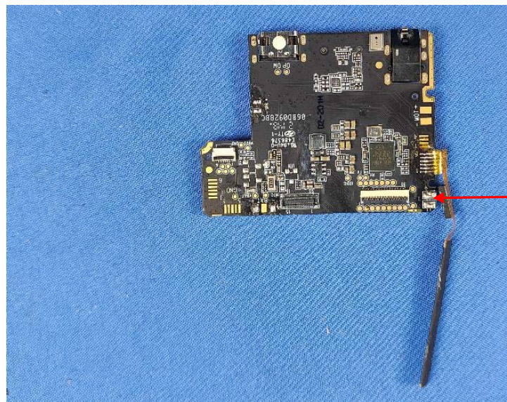
Bluetooth Antenna
