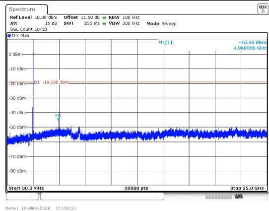
30.0 MHz - 25000.0 MHz 2.4G_Channel 39
