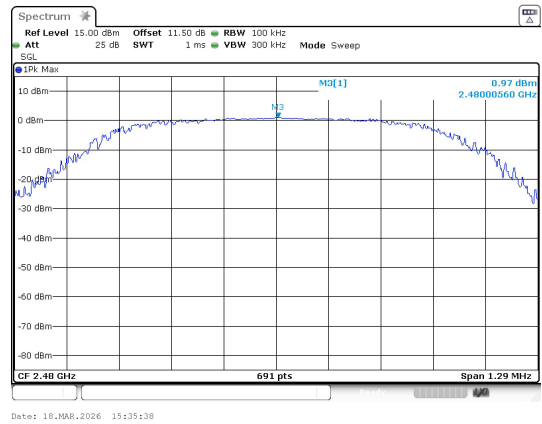
In-Band Reference Level 2.4G_Channel 39
