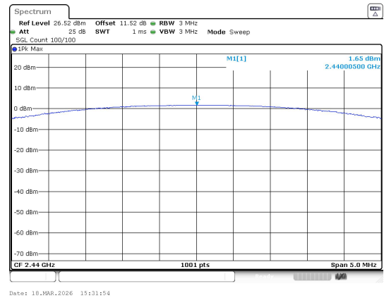
Peak Output Power 2.4G_Channel 19
