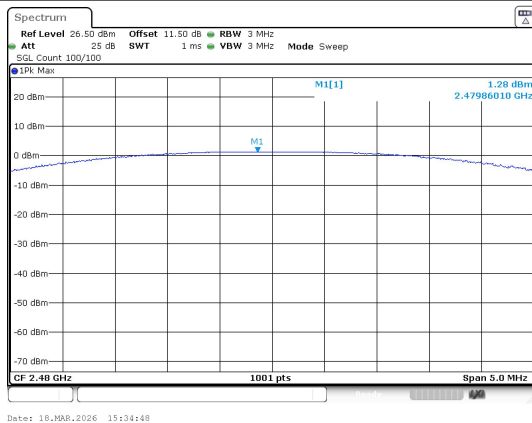
Peak Output Power 2.4G_Channel 39
