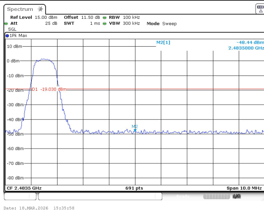
Out Of Band Emission 2.4G_Channel 39
