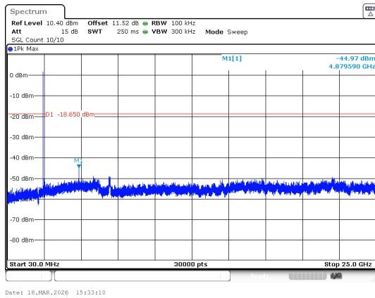
30.0 MHz - 25000.0 MHz 2.4G_Channel 19
