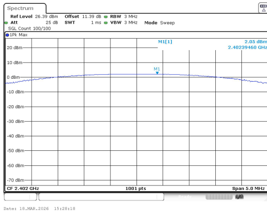
Peak Output Power 2.4G_Channel 0
