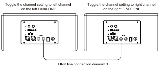
LINK line connection diagram 1
