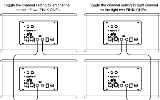
LINK line connection diagram 2
