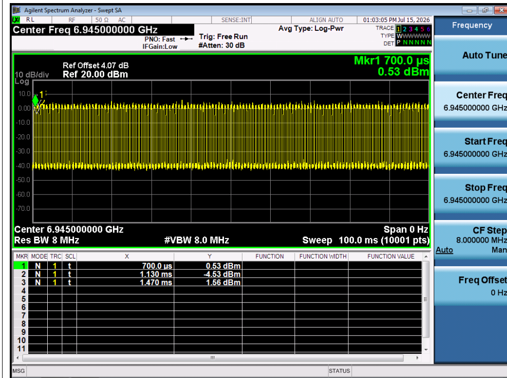
Duty Cycle NVNT be80 6945MHz AntA
