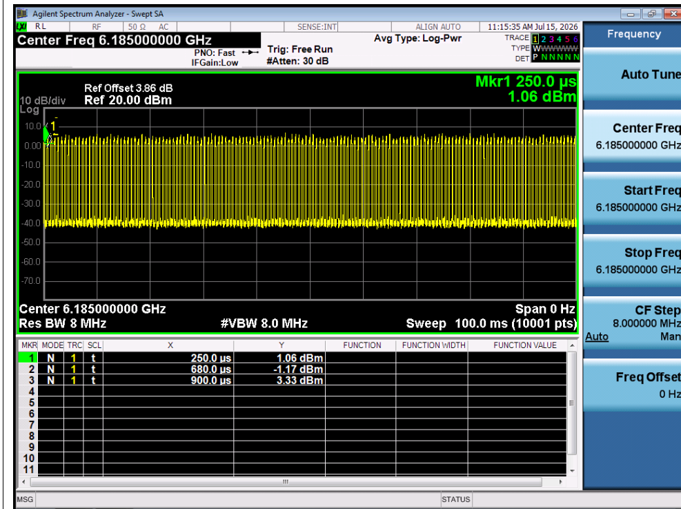
Duty Cycle NVNT be160 6185MHz AntB
