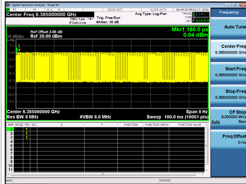
Duty Cycle NVNT be80 6385MHz AntB
