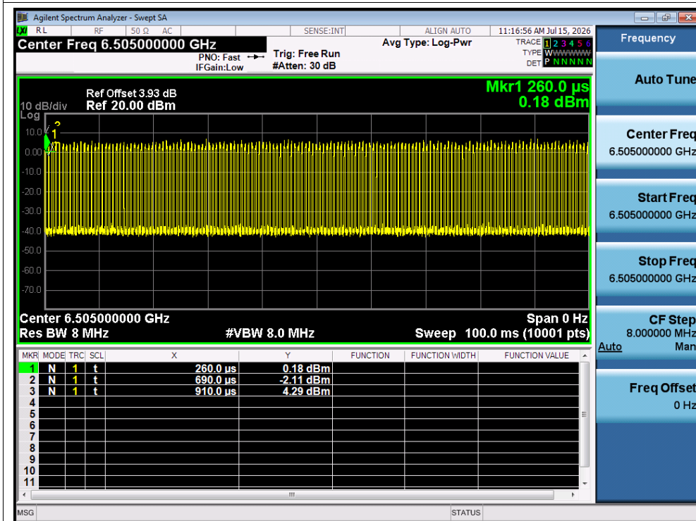
Duty Cycle NVNT be160 6505MHz AntB
