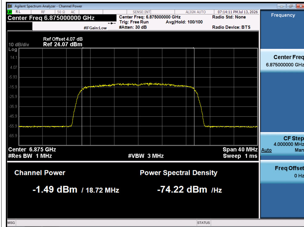
Power NVNT be20 6875MHz AntB
