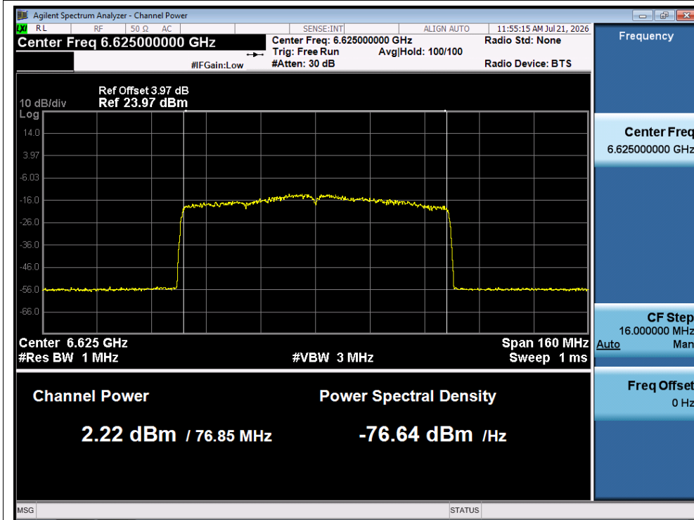
Power NVNT ax80 6625MHz AntB
