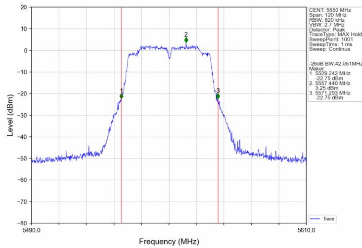
802.11ac(VHT40)_MCH_5550MHz_Ant1_NTNV
