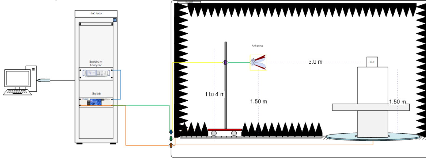
Radiated Setup 1 GHz – 6.4 GHz
