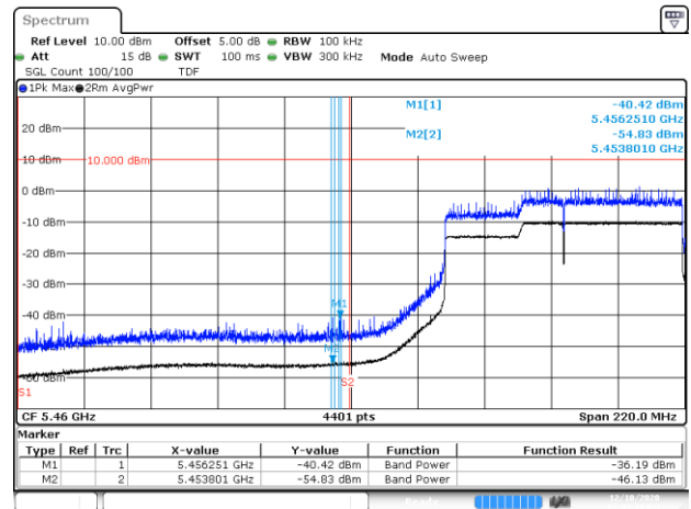
BE-R-LOW, MIMO-B, 802.11ax160-HE0, Ch114
