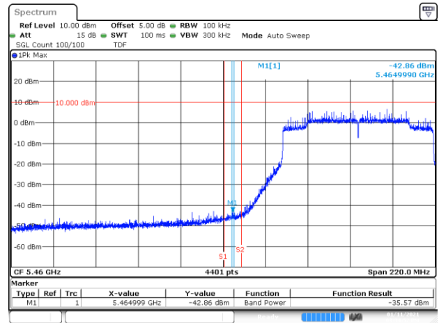
BE-NR-LOW, MIMO-B, 802.11ax80-HE0, Ch106
