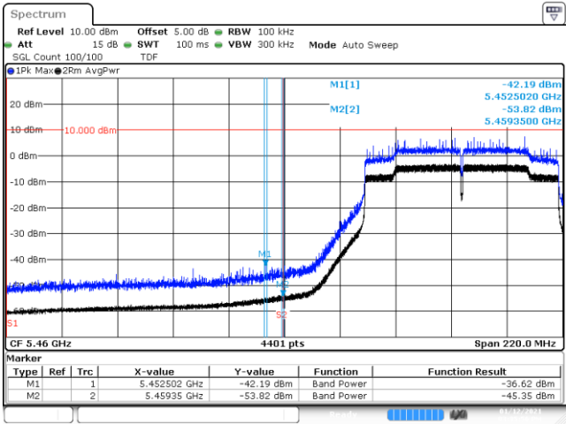
BE-R-LOW, MIMO-A, 802.11ac80-VHT0, Ch106
