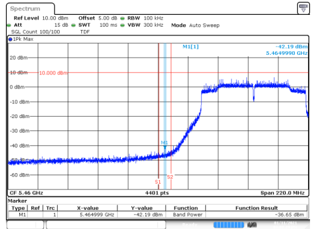
BE-NR-LOW, MIMO-B, 802.11ac80-VHT0, Ch106
