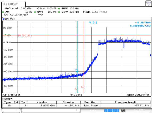
BE-NR-LOW, MIMO-A, 802.11ac80-VHT0, Ch106
