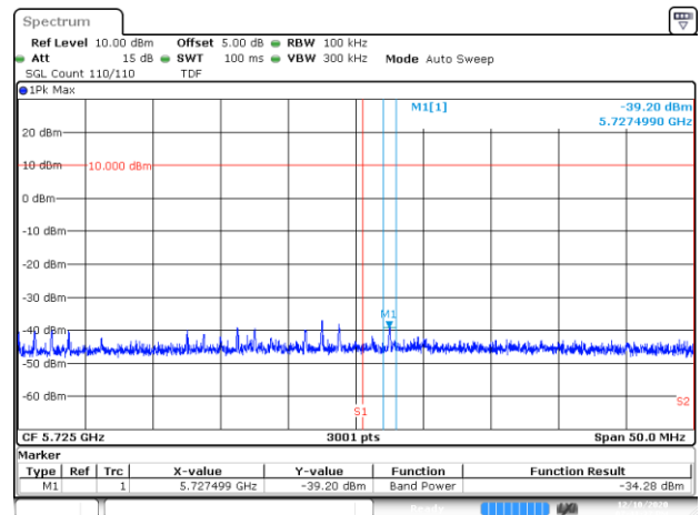
BE-NR-HIGH, MIMO-B, 802.11ax160-HE0, Ch114
