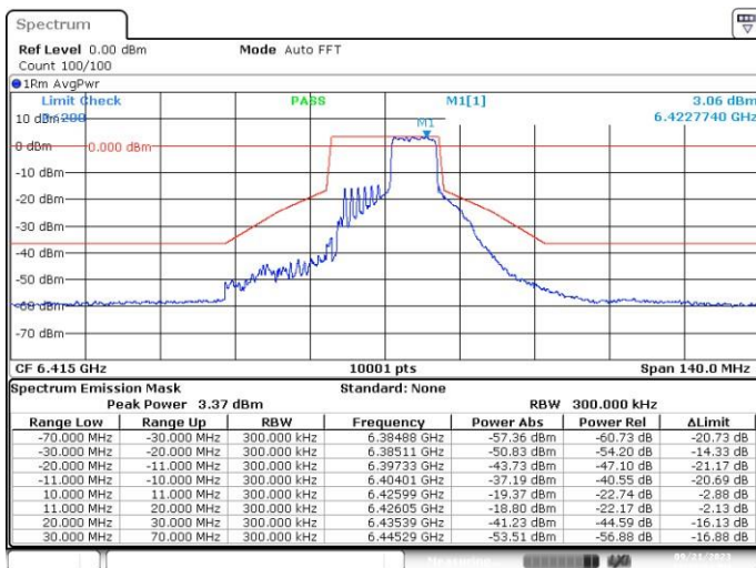
MIMO-B, 802.11ax/be20-MCS0, Ch93-8m-53
