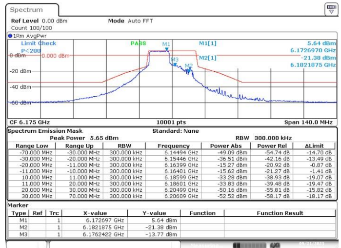
SISO-B, 802.11ax/be20-MCS0, Ch45-8m-53
