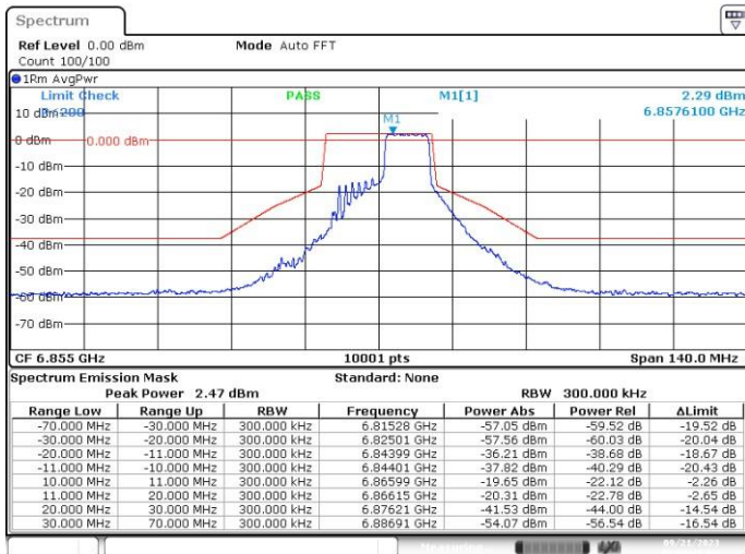
MIMO-A, 802.11ax/be20-MCS0, Ch181-8m-53
