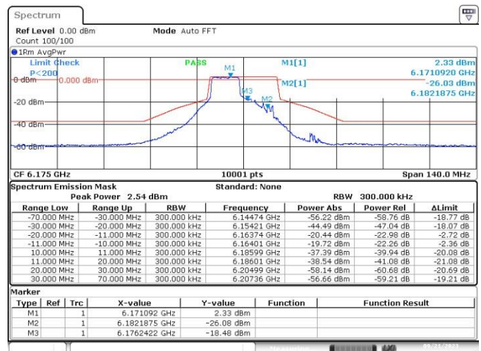
MIMO-A, 802.11ax/be20-MCS0, Ch45-8m-53
