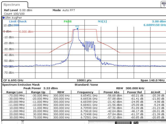
MIMO-A, 802.11ax/be20-MCS0, Ch149-4m-37
