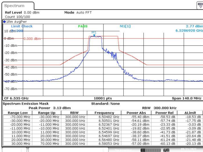
MIMO-A, 802.11ax/be20-MCS0, Ch117-8m-53
