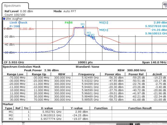
MIMO-B, 802.11ax/be20-MCS0, Ch1-8m-53
