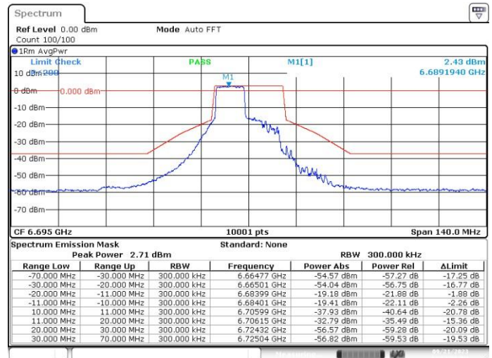
MIMO-A, 802.11ax/be20-MCS0, Ch149-8m-53
