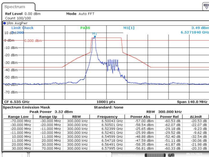
MIMO-A, 802.11ax/be20-MCS0, Ch117-2m-0
