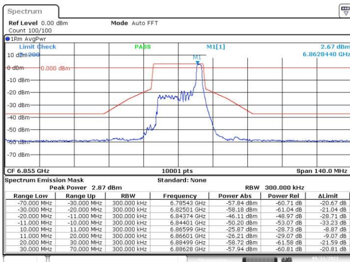
MIMO-A, 802.11ax/be20-MCS0, Ch181-2m-0
