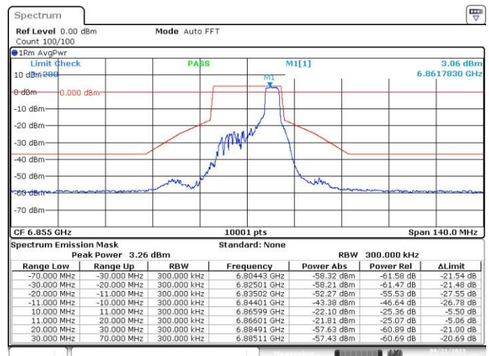
MIMO-A, 802.11ax/be20-MCS0, Ch181-4m-37
