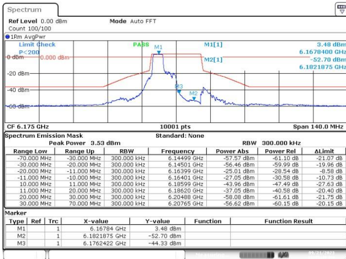
MIMO-B, 802.11ax/be20-MCS0, Ch45-4m-37
