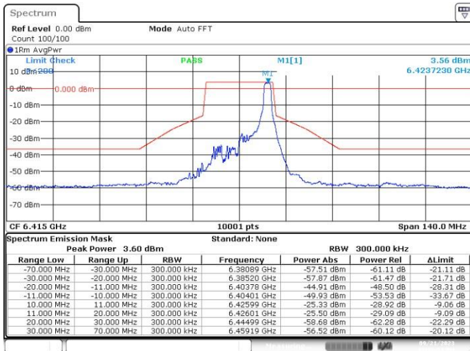
MIMO-B, 802.11ax/be20-MCS0, Ch93-2m-0
