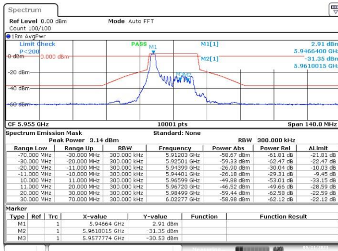
MIMO-B, 802.11ax/be20-MCS0, Ch1-2m-0
