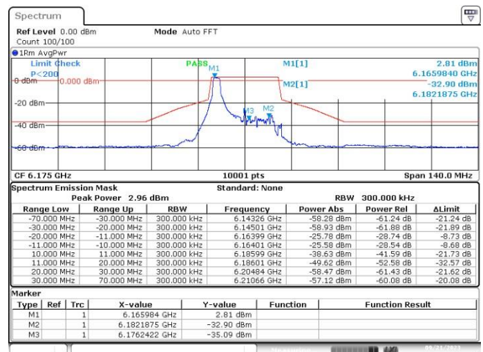
MIMO-B, 802.11ax/be20-MCS0, Ch45-2m-0
