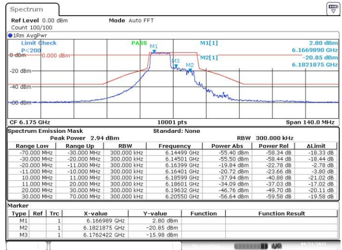
MIMO-B, 802.11ax/be20-MCS0, Ch45-8m-53
