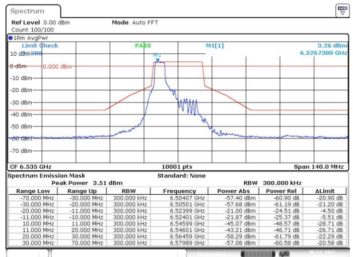
MIMO-A, 802.11ax/be20-MCS0, Ch117-4m-37
