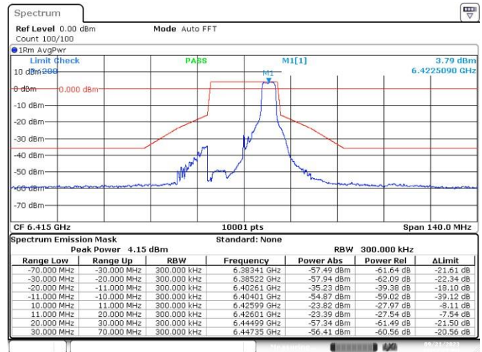
MIMO-B, 802.11ax/be20-MCS0, Ch93-4m-37
