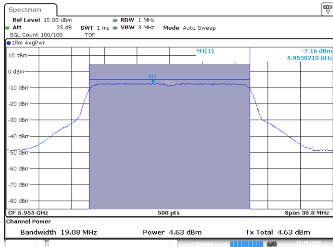
SISO B-802.11ax-20MHz-Ch1-5955MHz-HE0
