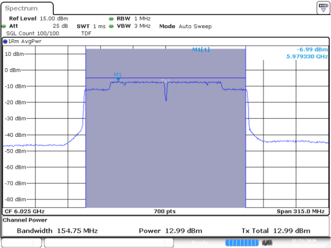
SISO A-802.11ax-160MHz-Ch15-6025MHz-HE0
