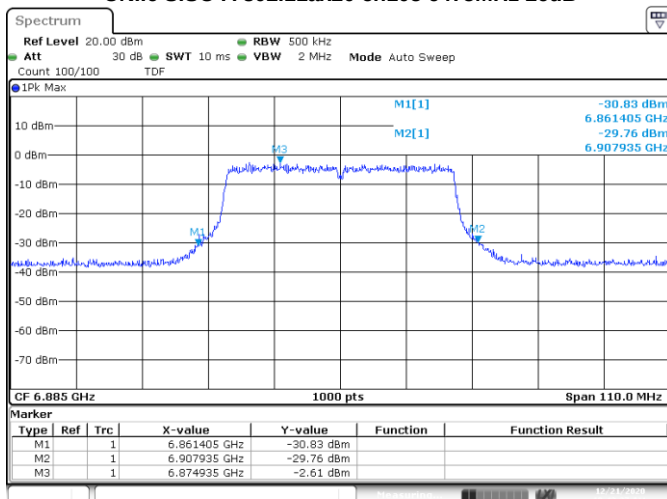
UNII8 SISO A 802.11ax40 ch187 6885MHz 26dB
