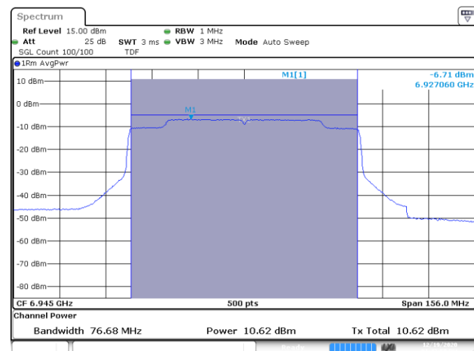
SISO B-802.11ax-80MHz-Ch199-6945MHz-HE0
