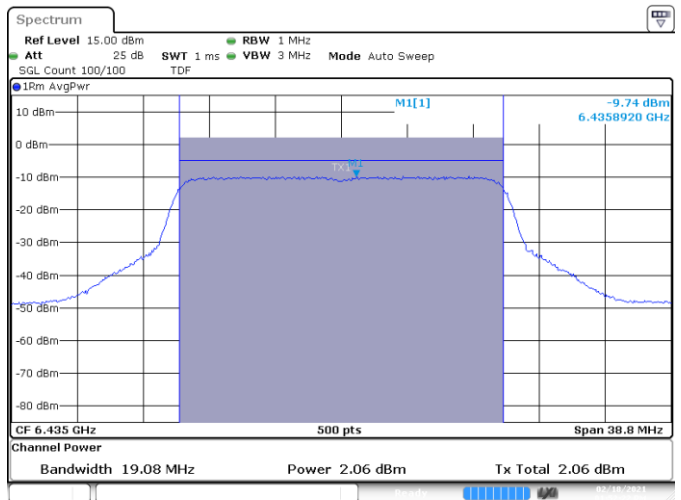
MIMO B-802.11ax-20MHz-Ch97-6435MHz-HE0
