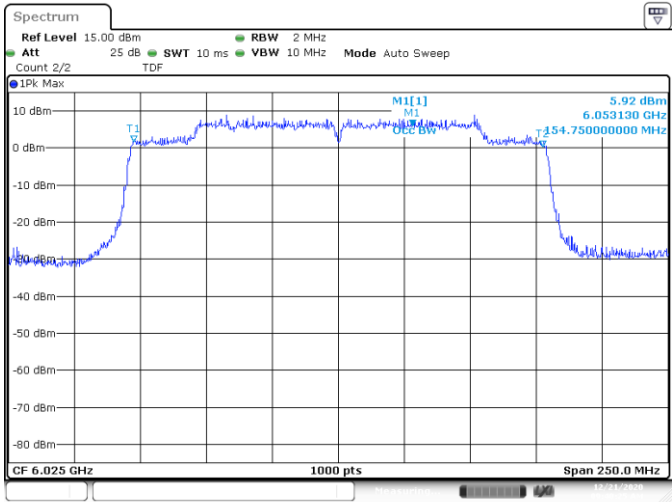
UNII5 SISO A 802.11ax160 ch15 6025MHz 99%
