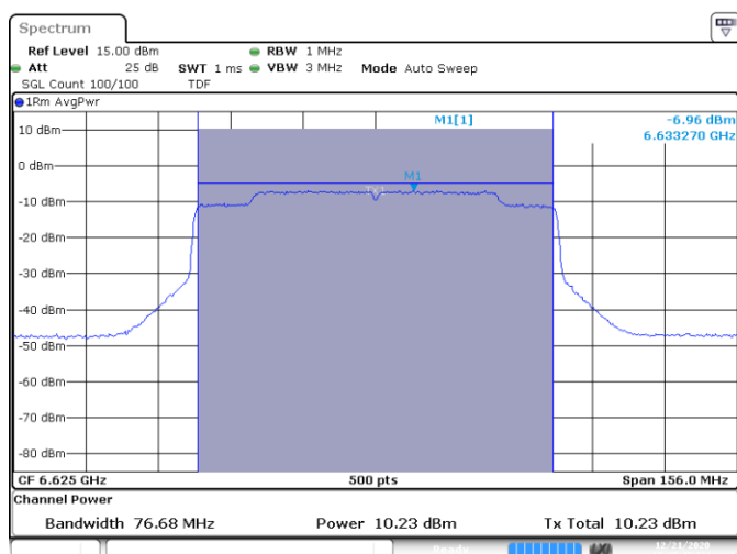
SISO A-802.11ax-80MHz-Ch135-6625MHz-HE0
