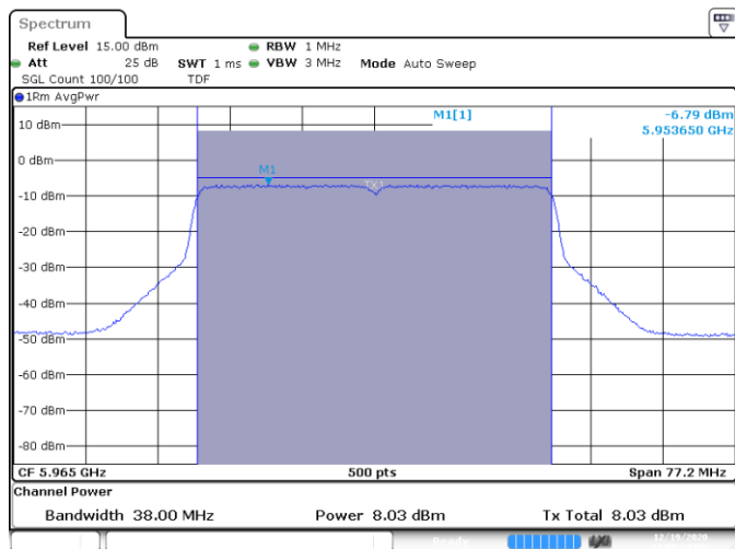
SISO B-802.11ax-40MHz-Ch3-5965MHz-HE0
