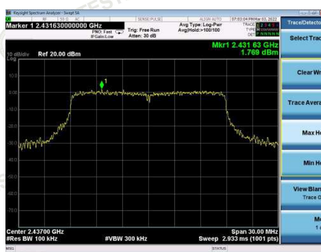
Reference CH06
