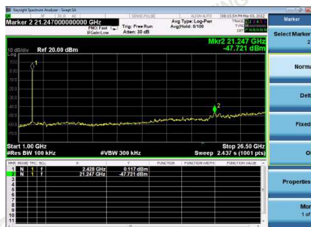
1GHz-26.5GHz
