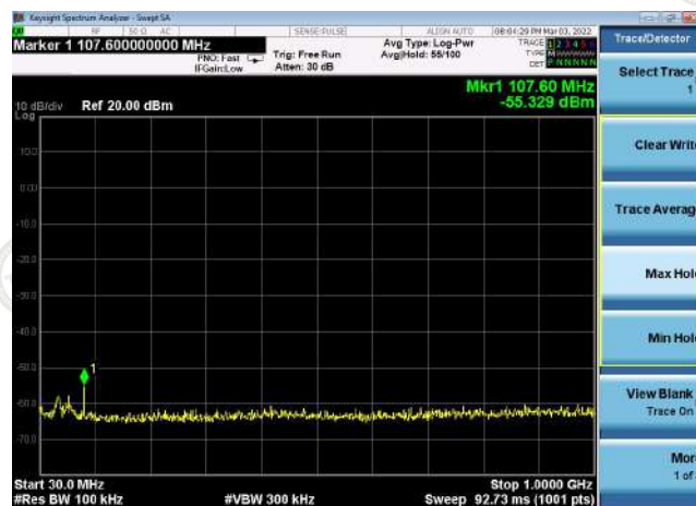
30MHz-1GHz
