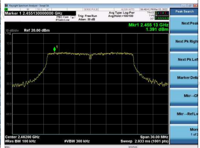
Reference CH11
