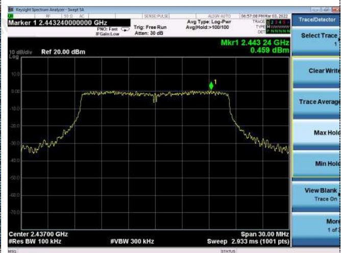
Reference CH06
