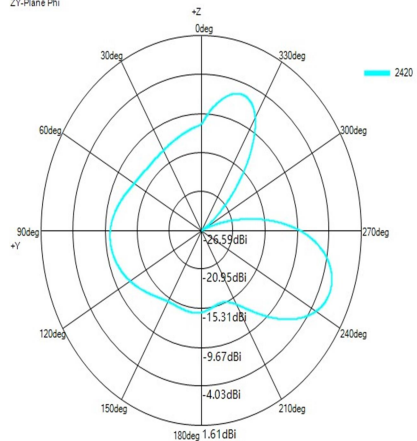
ZY-Plane Phi
