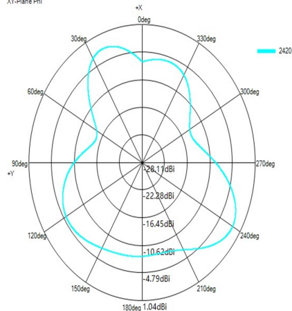
XY-Plane Phi
