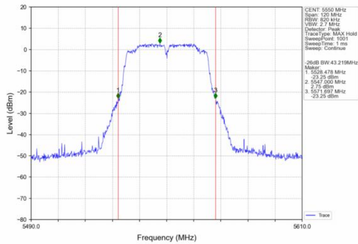
802.11n(HT40)_MCH_5550MHz_Ant1_NTNV
