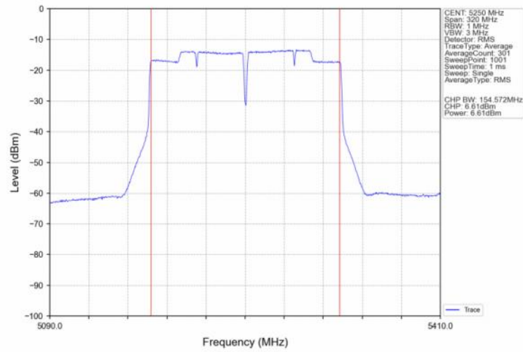
802.11ac(VHT160)_MCH_5250MHz_Ant2_NTNV
