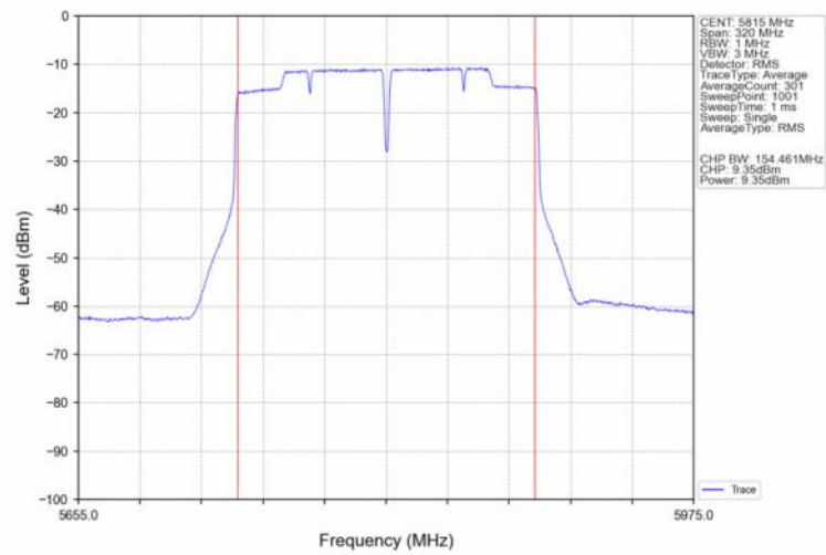
802.11ac(VHT160) HCH_5815MHz_Ant2_NTNV
