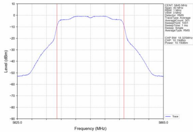
802.11ac(VHT20)_HCH_5845MHz_Ant2_NTNV
