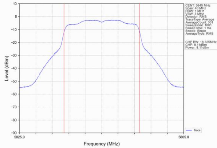
802.11ac(VHT20)_HCH_5845MHz_Ant2_NTNV
