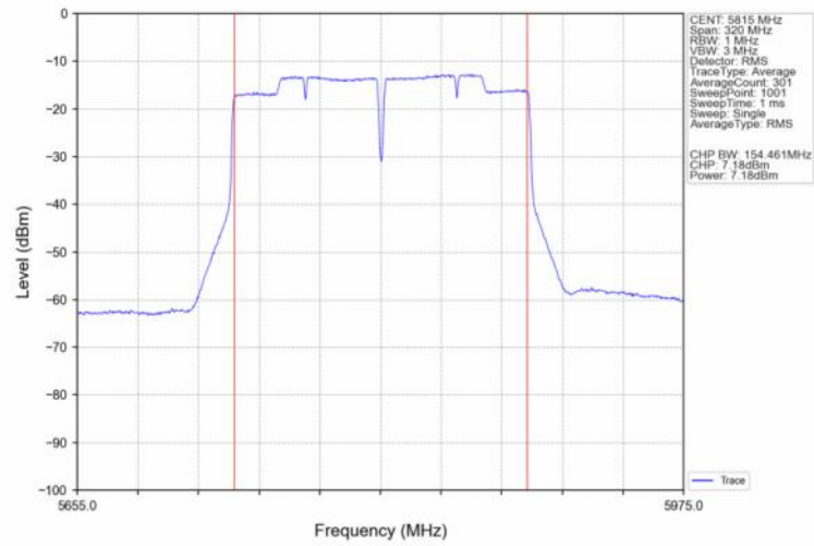
802.11ac(VHT160) HCH_5815MHz_Ant2_NTNV
