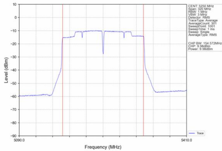
802.11ac(VHT160)_MCH_5250MHz_Ant2_NTNV
