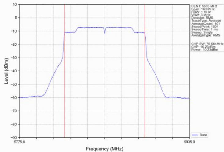
802.11ac(VHT80)_HCH_5855MHz_Ant2_NTNV
