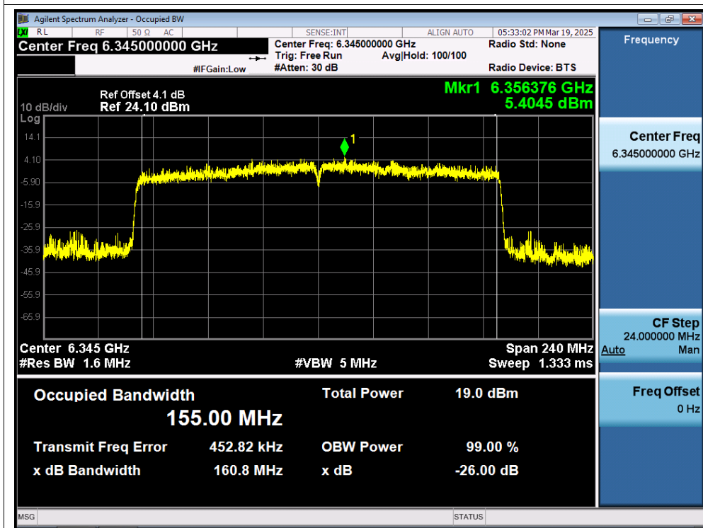
OBW NVNT ax160 6345MHz AntB
