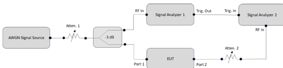
Figure 2. Contention-based protocol test setup, conducted method
