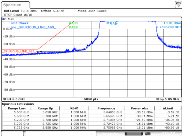
BE-NR-LOW, MIMO-B, 802.11ac80-HE0, Ch155
