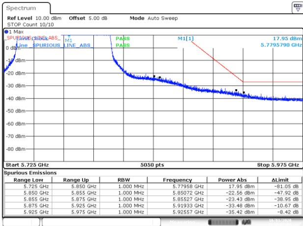
BE-NR-HIGH, MIMO-B, 802.11ac80-HE0, Ch155
