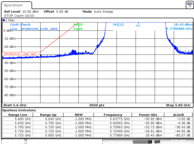
BE-NR-LOW, MIMO-A, 802.11ac80-HE0, Ch155
