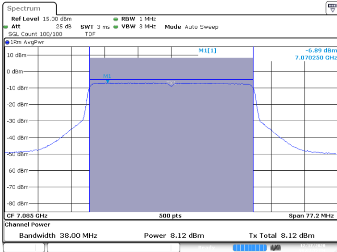
SISO B-802.11ax-40MHz-Ch227-7085MHz-HE0
