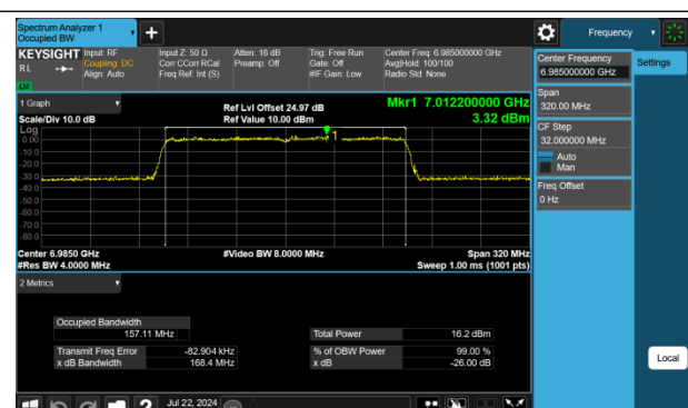
802.11ax-HE160 / CH207
