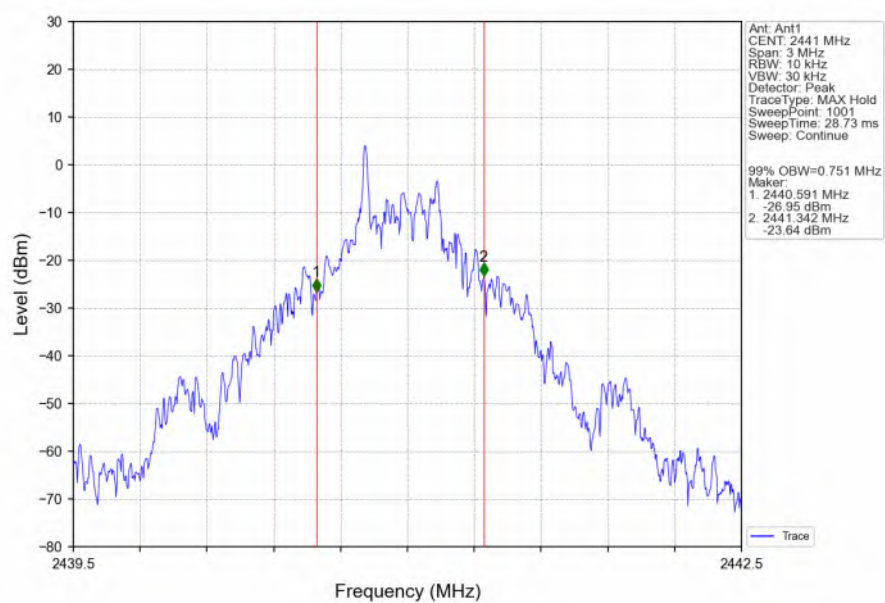
GFSK_DH5_MCH_2441MHz_Ant1_NTNV
