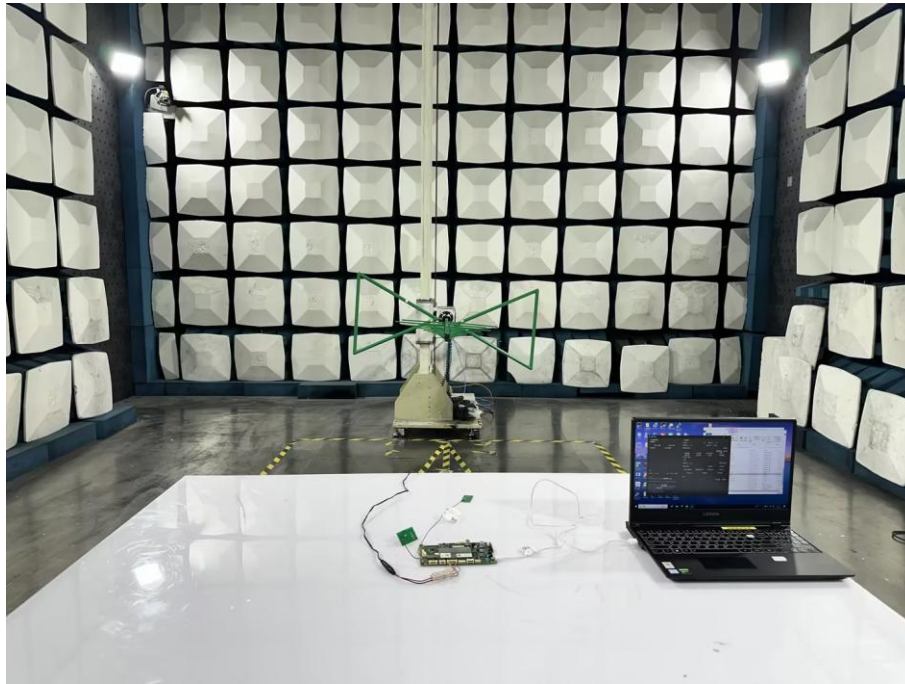
RF Radiated setup (30-1000MHz)
