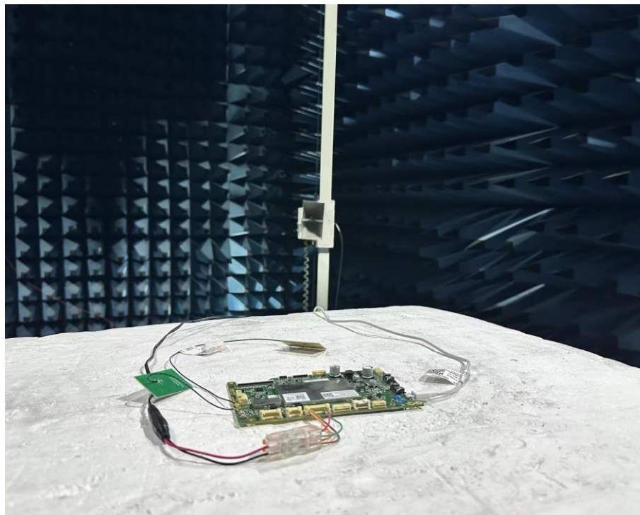
RF Radiated setup (1-18GHz)
