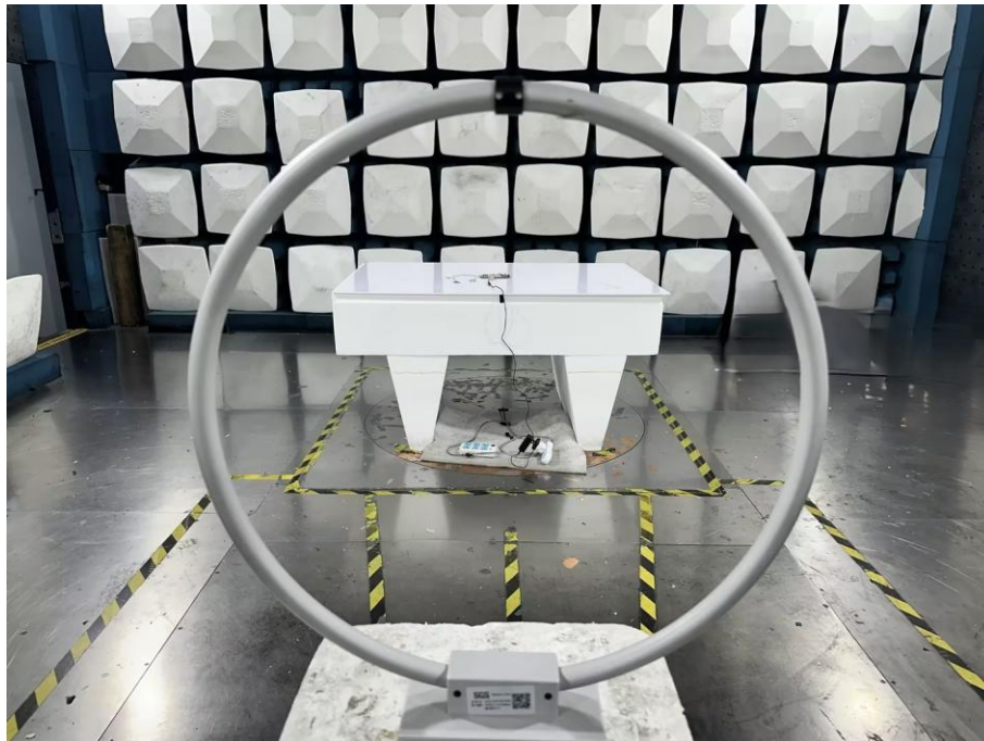
RF Radiated setup (9K-30MHz)
