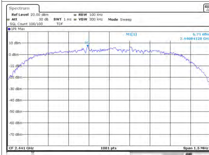
Tx. Spurious NVNT 2-DH5 2441MHz Ref
