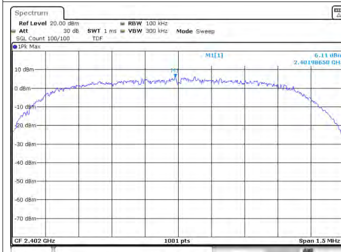
Tx. Spurious NVNT 2-DH5 2402MHz Ref
