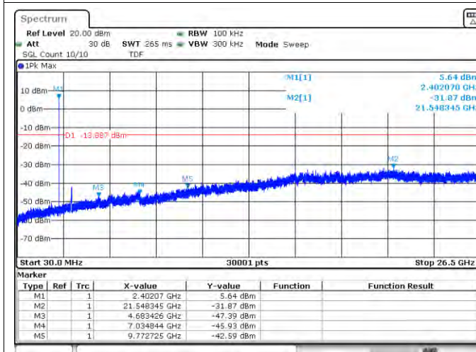
Tx. Spurious NVNT 2-DH5 2402MHz Emission
