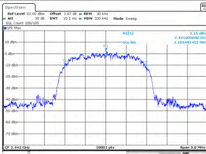
OBW NVNT 2-DH5 2441MHz
