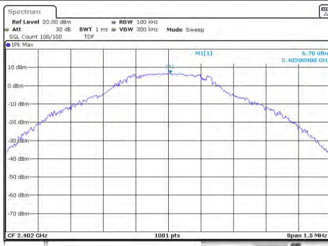
Tx. Spurious NVNT 1-DH5 2402MHz Ref
