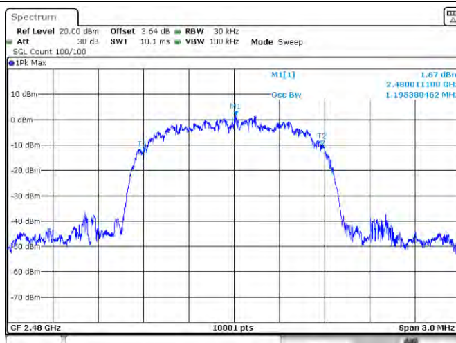
OBW NVNT 3-DH5 2480MHz
