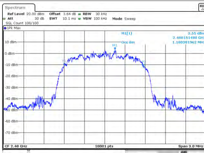
OBW NVNT 2-DH5 2480MHz
