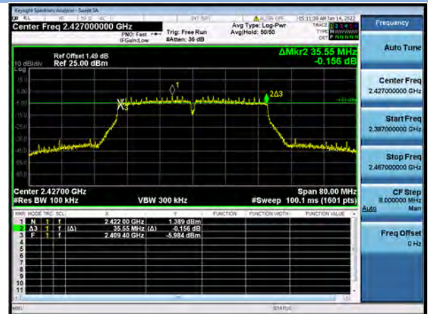
802.11n-40 MHz CHANNEL 4
