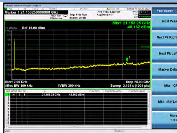
802.11b CHANNEL 13, SPURIOUS 2 GHz ~ 25 GHz
