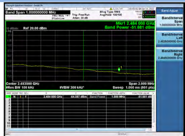
802.11n-20 MHz CHANNEL 13, Band Edge
