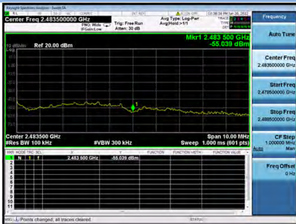
802.11b CHANNEL 12, Reference level
