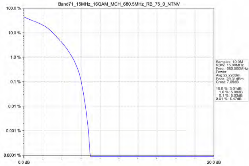
Band71_15MHz_16QAM_MCH_680.5MHz_RB_75_0_NTNV
