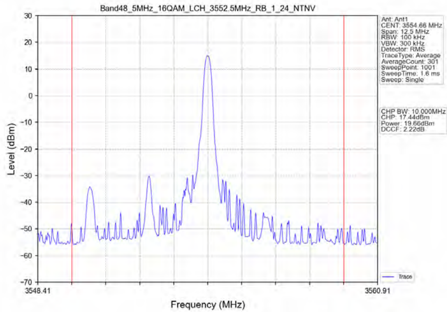
Band48 5MHz 16QAM LCH 3552.5MHz RB 1 24 NTN
