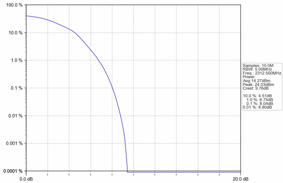
Band40a_5MHz_16QAM_HCH_2312.5MHz_RB_25_0_NTNV
