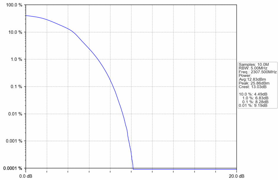
Band40a_5MHz_16QAM_LCH_2307.5MHz_RB_25_0_NTNV
