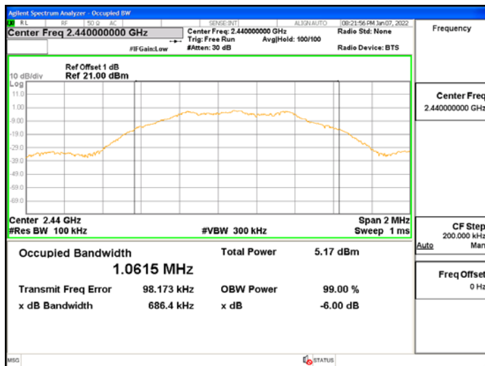
6dB BandwidthMode3 CH39
