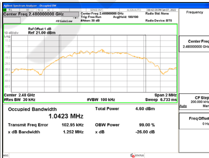
99% Bandwidth Mode3 CH39
