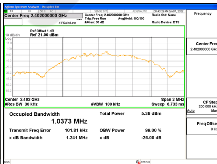
99% Bandwidth Mode1 CH00
