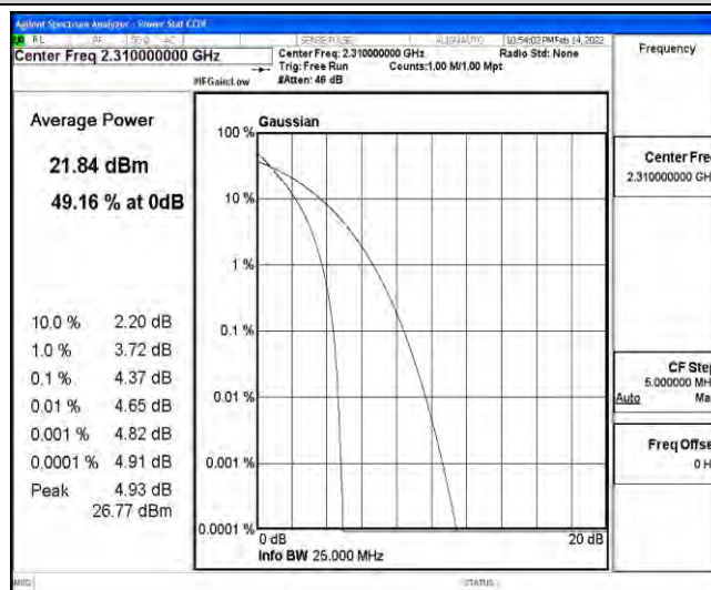
Band30-10MHz-16QAM-27710-1RB#0
