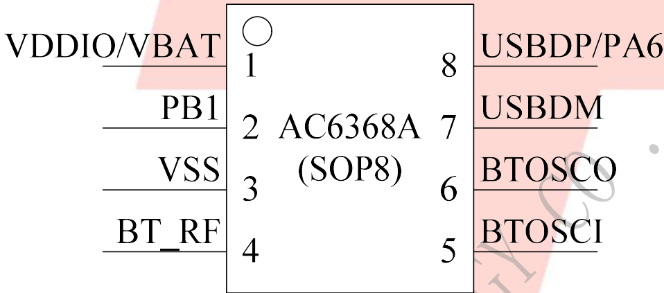
Figure 1-1 AC6368A Package Diagram
