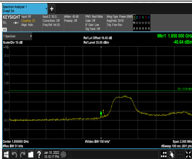
Band2-3MHz-16QAM-18615-1RB#14
