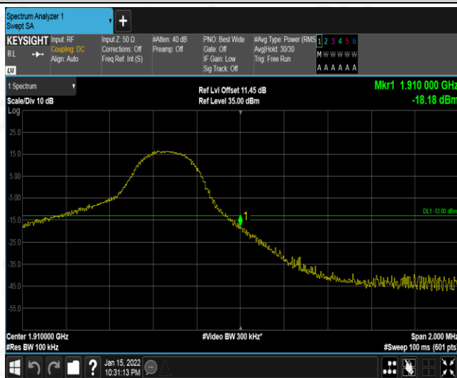
Band2-5MHz-16QAM-19175-1RB#24
