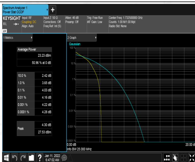
Band4-1.4MHz-QPSK-20175-6RB#0
