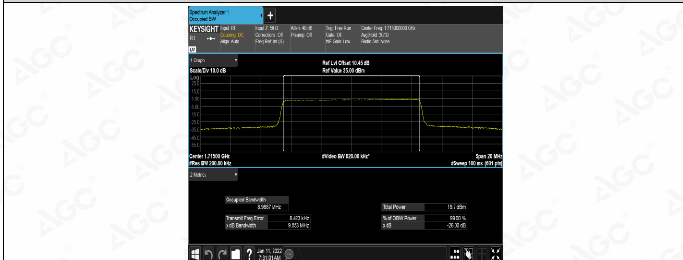
Band4-10MHz-QPSK-20175-50RB#0
