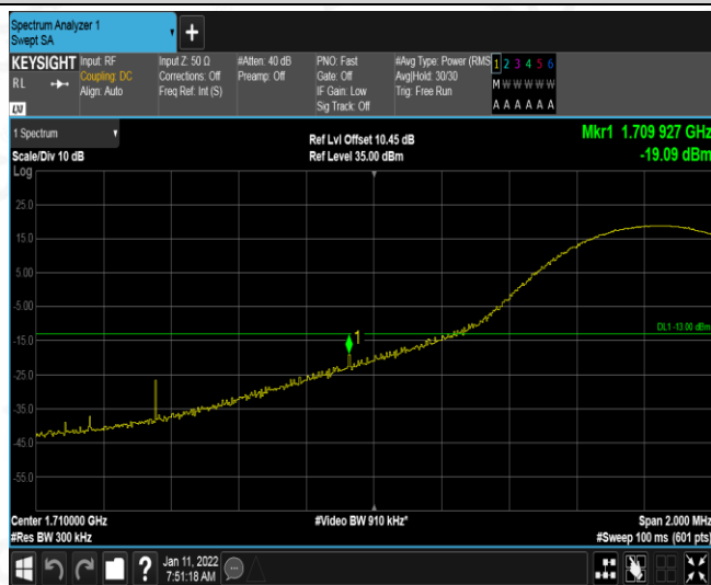
Band4-15MHz-QPSK-20025-1RB#74
