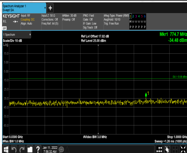
Band4-15MHz-16QAM-20025-1RB#0-Range1:30~1000MHz
