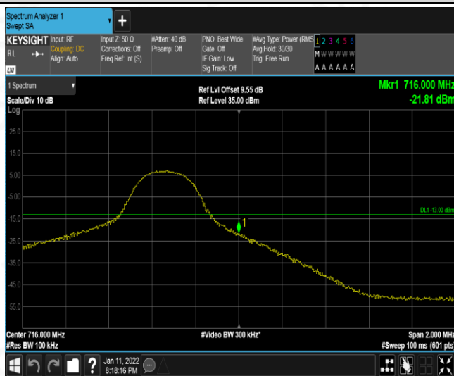
Band12-5MHz-QPSK-23155-1RB#24
