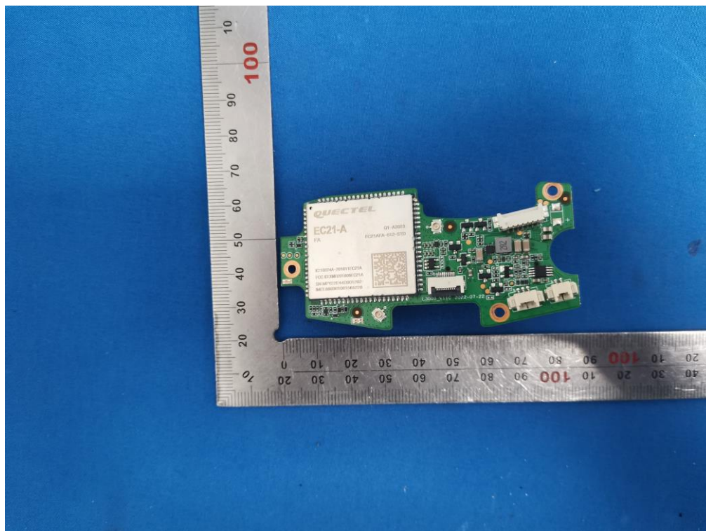
INTERNAL VIEW OF EUT(FIGURE 27)
