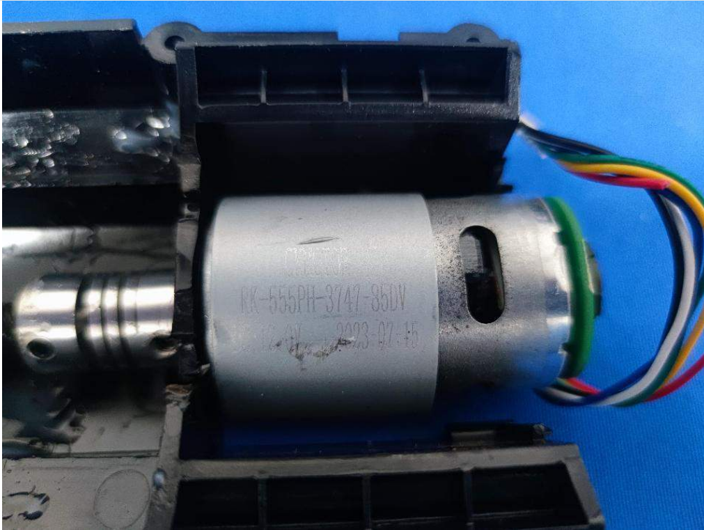
Motor(CK-RK-555PH-3747-85DV)
