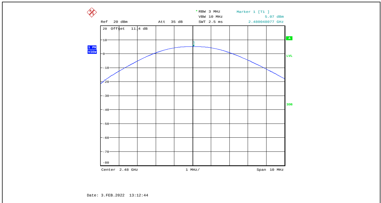
Plot 5.2.4.3. Maximum Peak Conducted Output Power, GFSK Modulation, 6 dBm Power Setting, 2480 MHz, 1 Mbps
