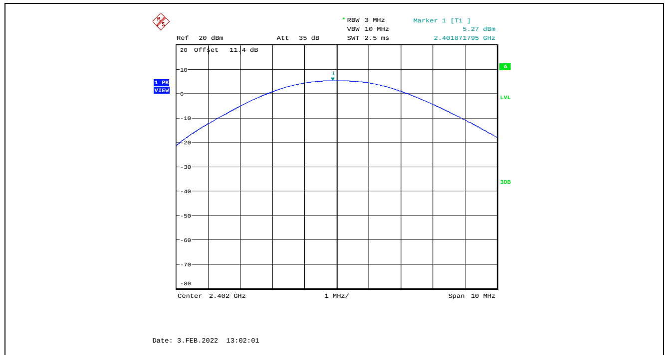
Plot 5.2.4.1. Maximum Peak Conducted Output Power, GFSK Modulation, 6 dBm Power Setting, 2402 MHz, 1 Mbps
