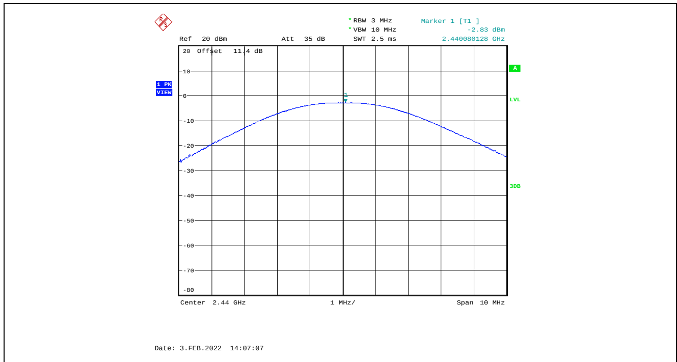
Plot 5.2.4.5. Maximum Peak Conducted Output Power, GFSK Modulation, -0.15 dBm Power Setting, 2440 MHz, 1 Mbps
