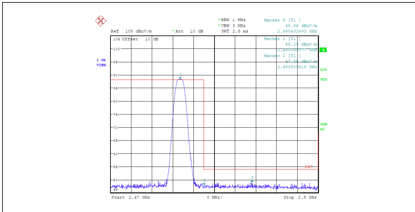
Plot 5.3.4.2.3. Band-Edge RF Radiated Emissions at 3 m, Vertical Polarization 2480 MHz, High End of Frequency Band
